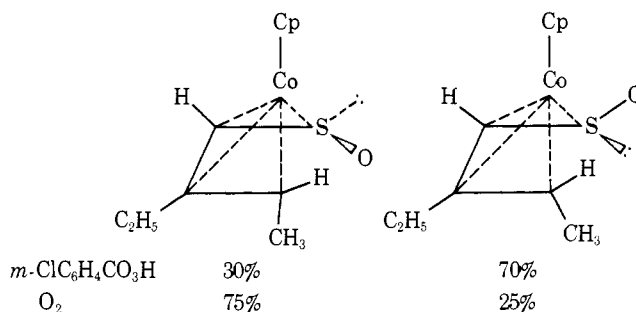
Figure 5. Relative amounts of S -oxide formed by oxidation of 12 with m -chloroperbenzoic acid and with air ( \text{Cp} = \pi\text{-C}_5\text{H}_5 ).
