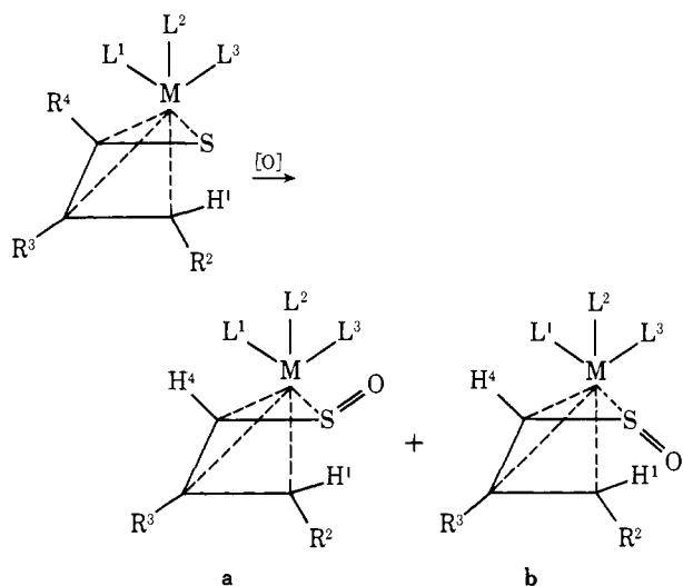
Figure 4. ^1\text{H} NMR chemical shifts for 18 ( \delta values in ppm downfield from internal tetramethylsilane).
