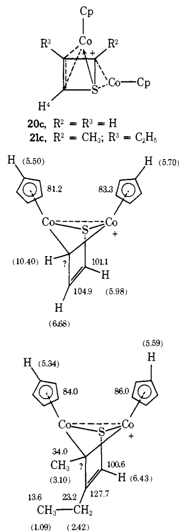
Figure 6. ^1H NMR and ^{13}C NMR chemical shifts (ppm downfield from Me_4Si ) for cobalt salts. ^1H NMR shifts are in parentheses.
