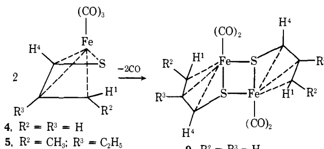
Figure 1. ^{13}\text{C} NMR chemical shifts ( \delta in ppm downfield from internal tetramethylsilane).
