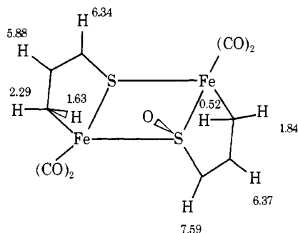
Figure 4. ^1\text{H} NMR chemical shifts for 18 ( \delta values in ppm downfield from internal tetramethylsilane).
