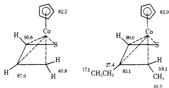
Figure 3. ^{13}\text{C} NMR chemical shifts ( \delta in ppm downfield from internal tetramethylsilane).
