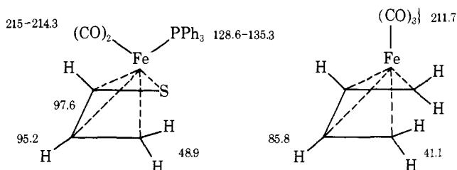
Figure 1. ^{13}\text{C} NMR chemical shifts ( \delta in ppm downfield from internal tetramethylsilane).
